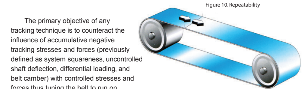
Figure 10. Repeatability
