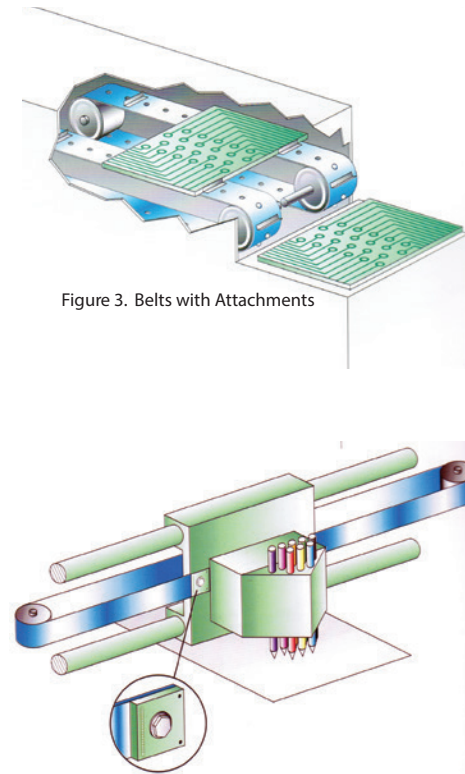
Figure 4. Drive Tapes
